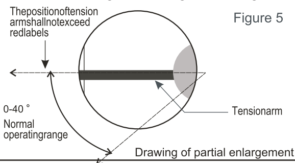
Partial enlarged drawing of warning line
